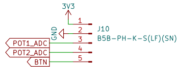
Controls Daughterboard
